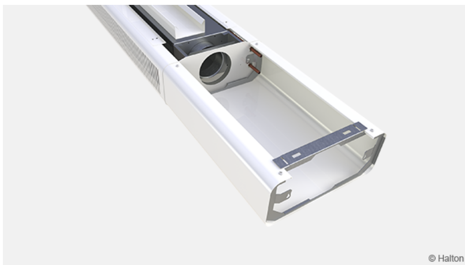
Fig. 20. Duct cover
