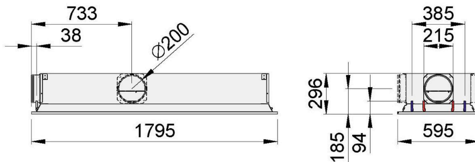
Fig. 29. Halton Rex RXP, Flexible and Autonomic models dimensions (RXP/S, RXP/F-1800 or RXP/A-1800)
