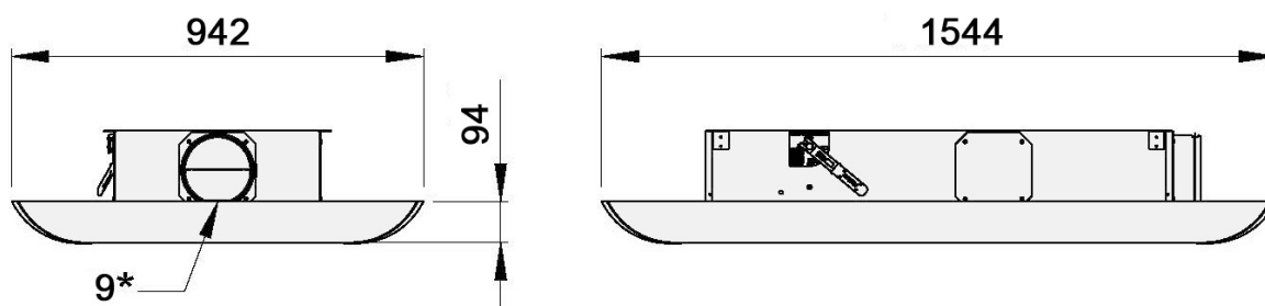
Fig. 31. Halton Rex RXP, Flexible and Autonomic models with Halton Coanda wings (RXP/S (with d125 and d160 duct connection), RXP/F-1200 or RXP/A-1200)
