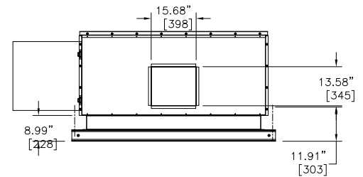
Right End View
