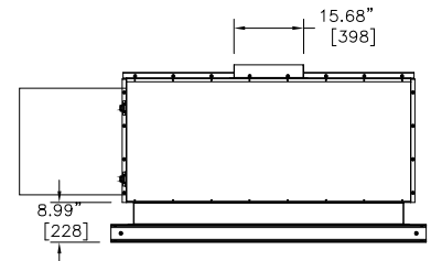
Right End View
