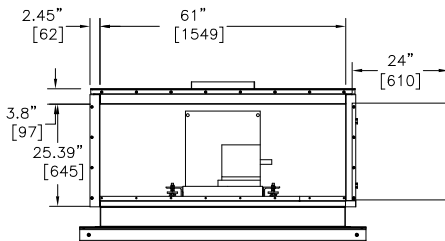
Left End View
