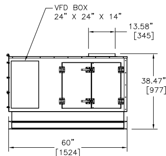
Right Hand Access Side Elevation
