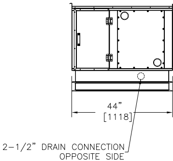
Right Hand Access Side Elevation
