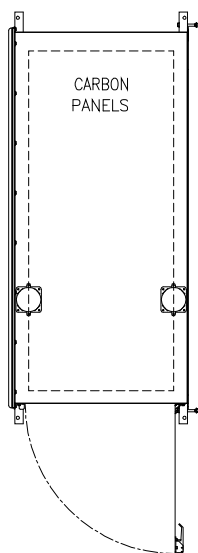
Plan View
