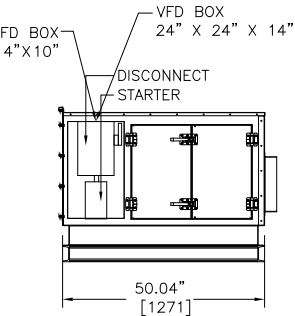
Right Hand Access Side Elevation
