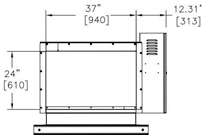
Left End View
