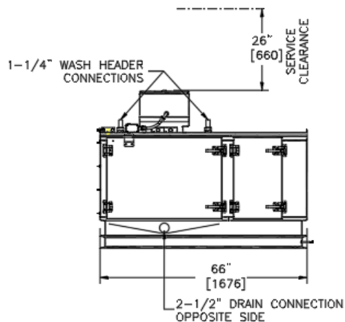
Right Hand Access Side Elevation
