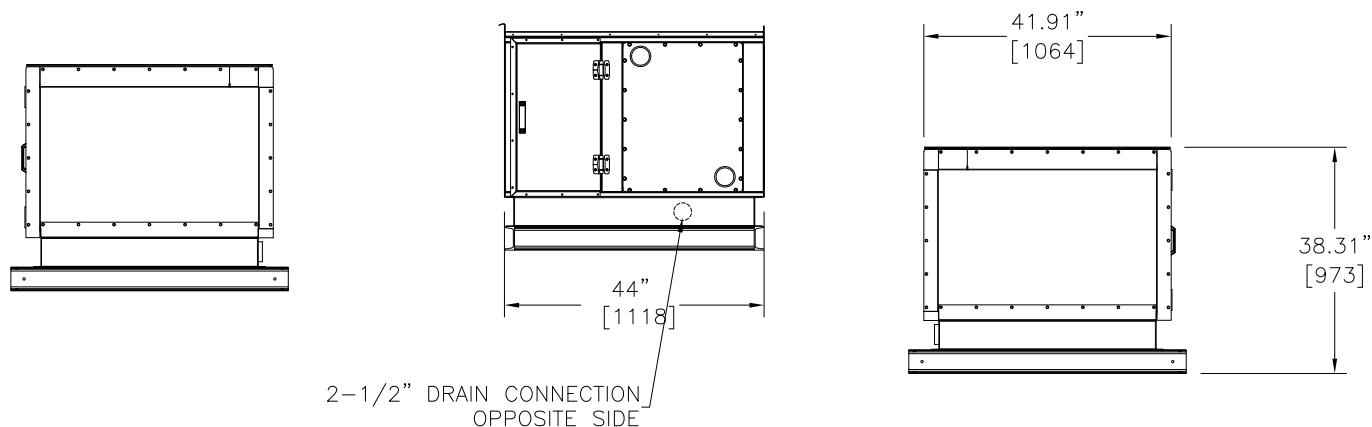
Left End View
