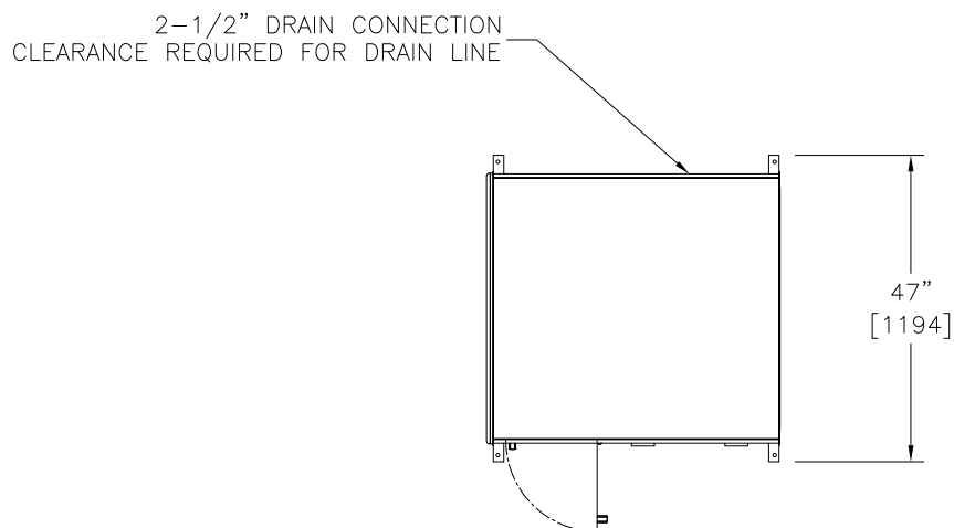
Plan View
