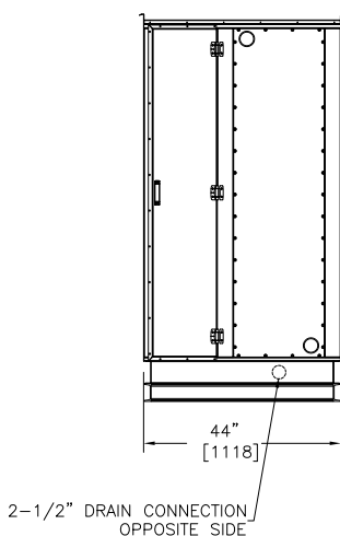
Right Hand Access Side Elevation
