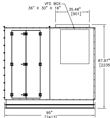
Right Hand Access Side Elevation
