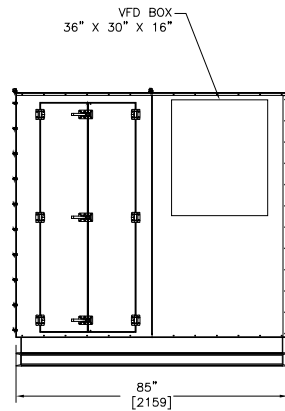
Right Hand Access Side Elevation
