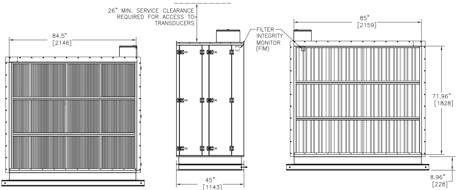
Right Hand Access Side Elevation
