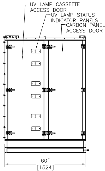
Right Hand Access Side Elevation
