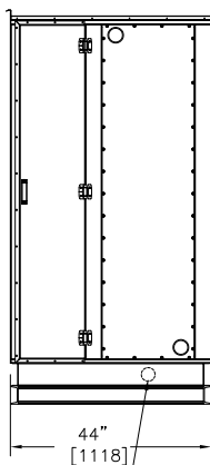
Right Hand Access Side Elevation
