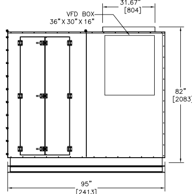
Right Hand Access Side Elevation
