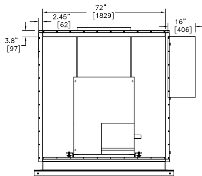
Left End View
