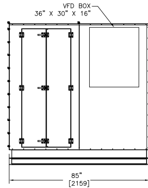
Right Hand Access Side Elevation
