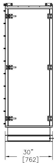
Right Hand Access Side Elevation
