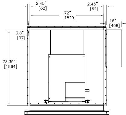
Left End View
