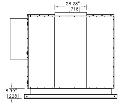
Right End View
