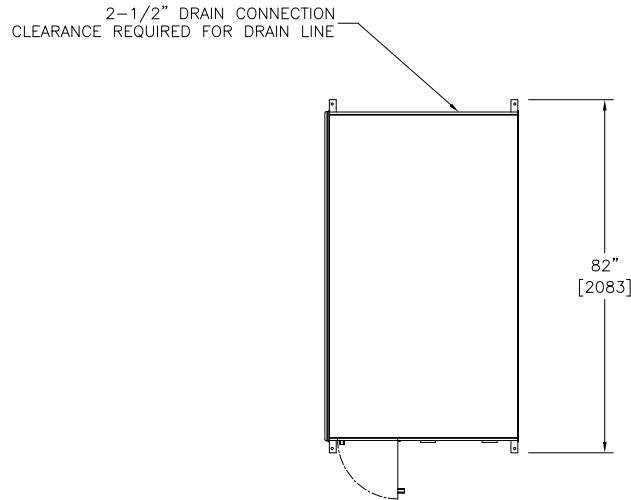
Plan View
