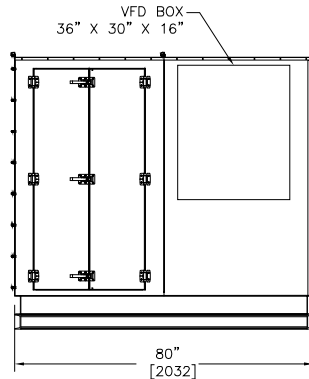
Right Hand Access Side Elevation
