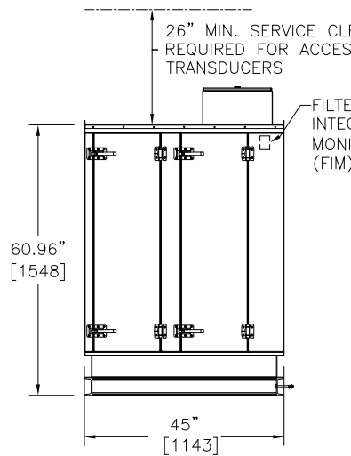
Right Hand Access Side Elevation
